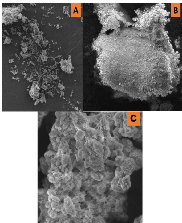
Figure 1: SEM images of (a) bare AgNPs, (b) FA capped AgNPs, and (c) HA capped AgNPs
