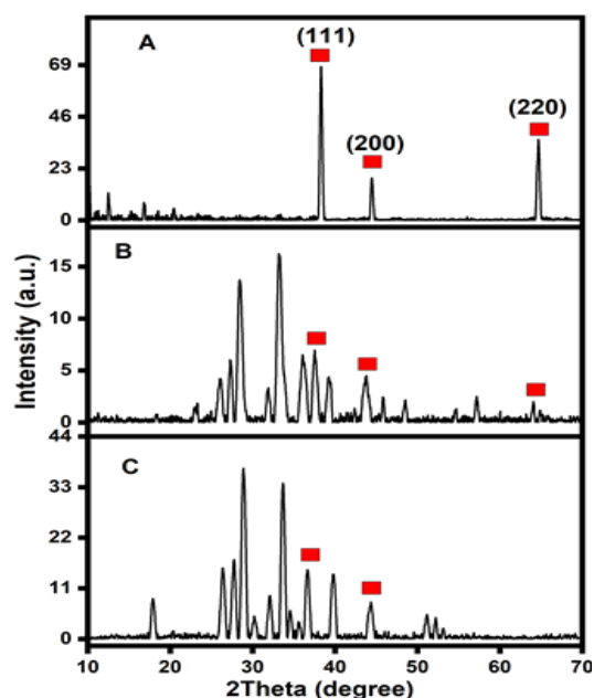
Figure 3: XRD pattern of (a) bare AgNPs, (b) FA capped AgNPs, and (c) HA capped AgNPs
